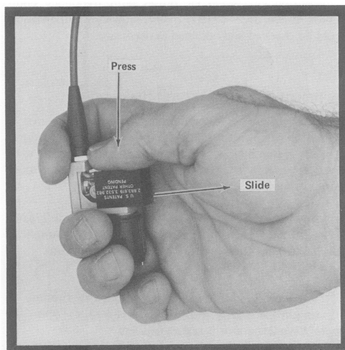
Fig. 6. Removal of compensation box cover.
