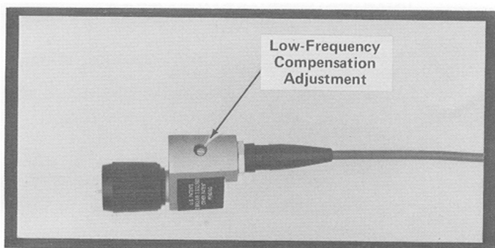
Fig. 7. Location of probe low-frequency compensation adjustment.
