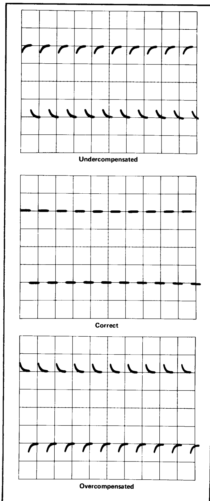
Fig. 8. Probe low-frequency compensation.
