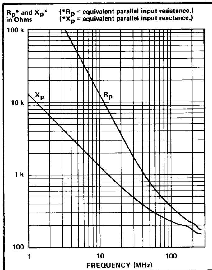
Fig. 3. P6053B Probe (6-foot cable), typical X_p , R_p versus frequency curves.
